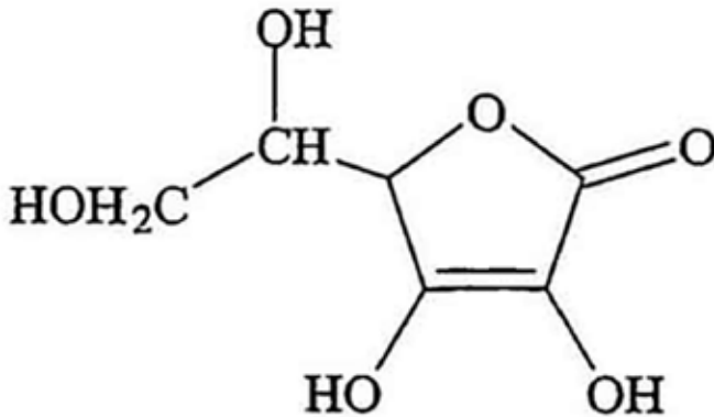
Ascorbic Acid
